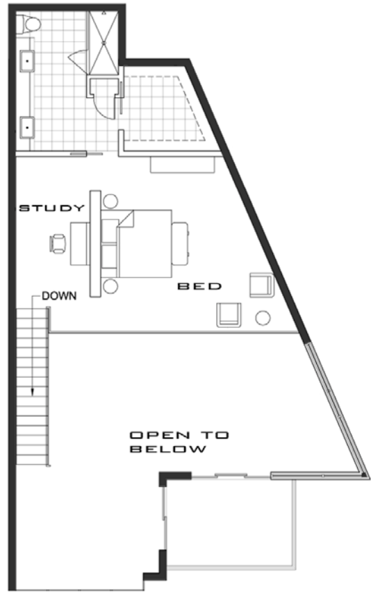
TYPE D SECOND FLOOR PLAN
