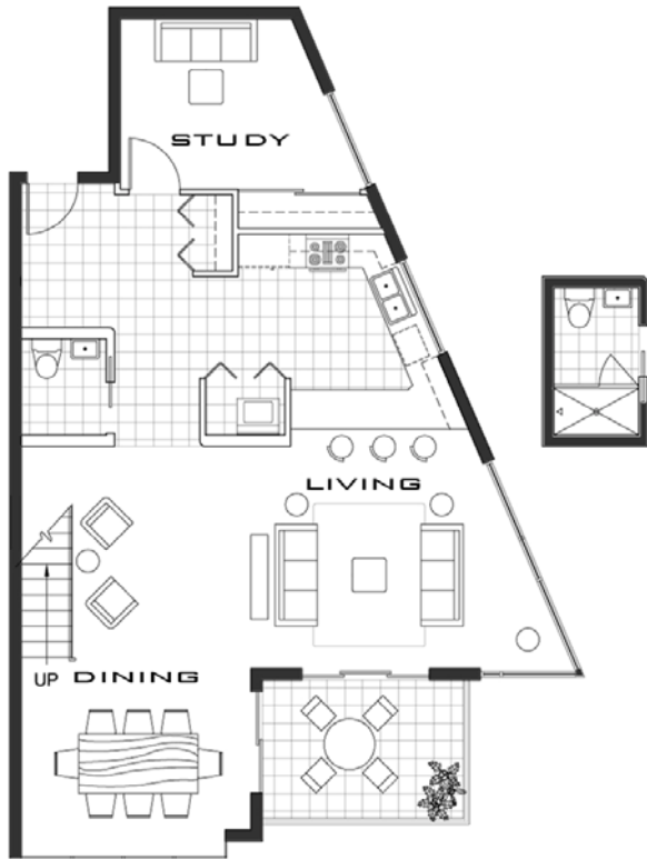
TYPE D FIRST FLOOR PLAN 1718 TOTAL SQ. FT.
