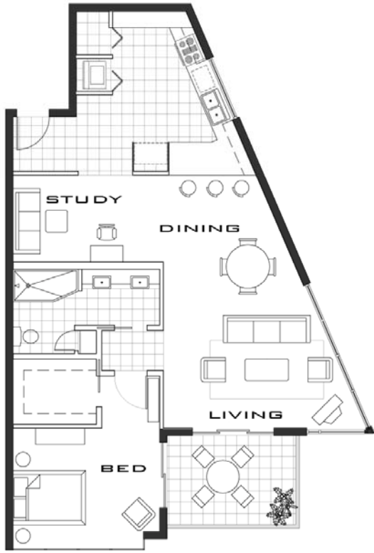
TYPE A FLOOR PLAN 1093 SQ. FT.
