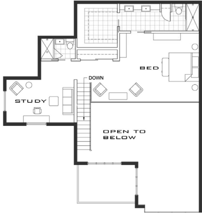
TYPE G SECOND FLOOR PLAN
